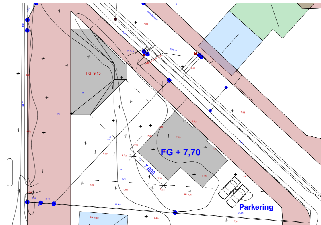
Situationsplan 1:400
